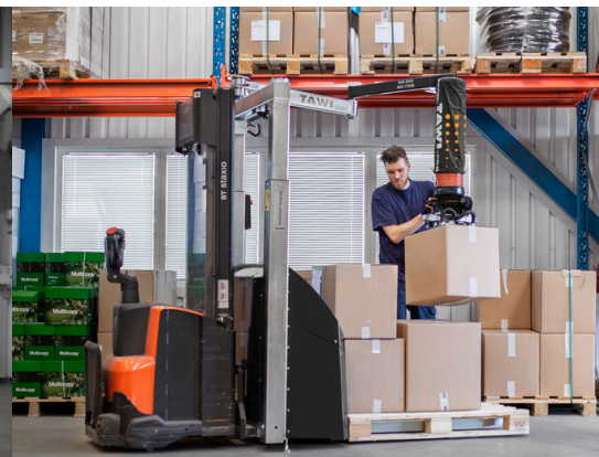
Mobile lifter
